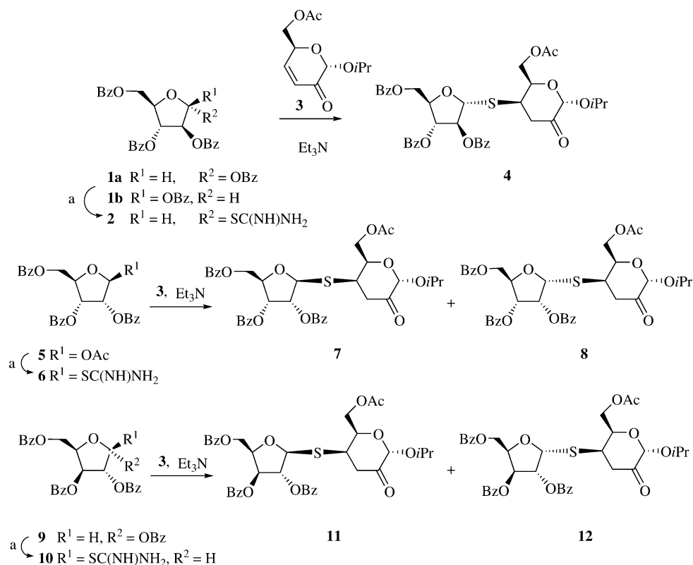
Scheme 1. Reaction conditions: (a) (\text{NH}_2)_2\text{CS} , \text{BF}_3 \cdot \text{OEt}_2 , \text{CH}_3\text{CN} , reflux.
